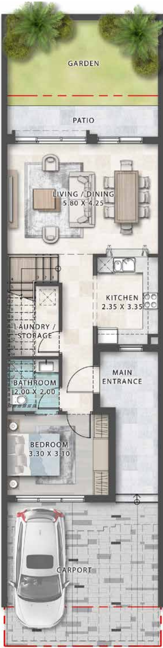
PIANO TERRA
